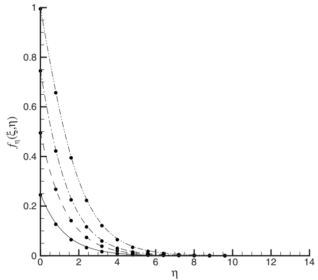
Fig. 4 The curves of f_{\eta}(\xi, \eta) in the case of \lambda=1/2 by means of \hbar=-1/5 . Solid line: \xi=1/4 , dashed line: \xi=1/2 , dash-dotted line: \xi=3/4 , and symbols: numerical results.
